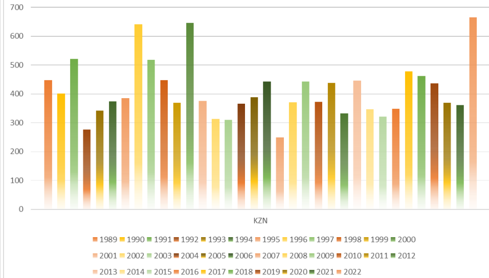
RAINFALL YEAR TO DATE KZN
