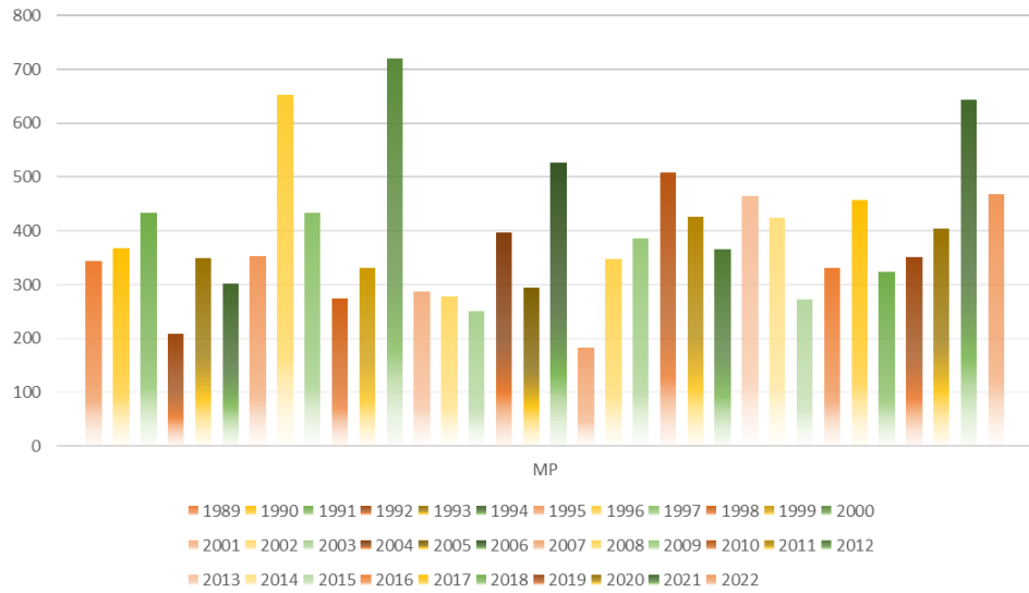
RAINFALL YEAR TO DATE MP
