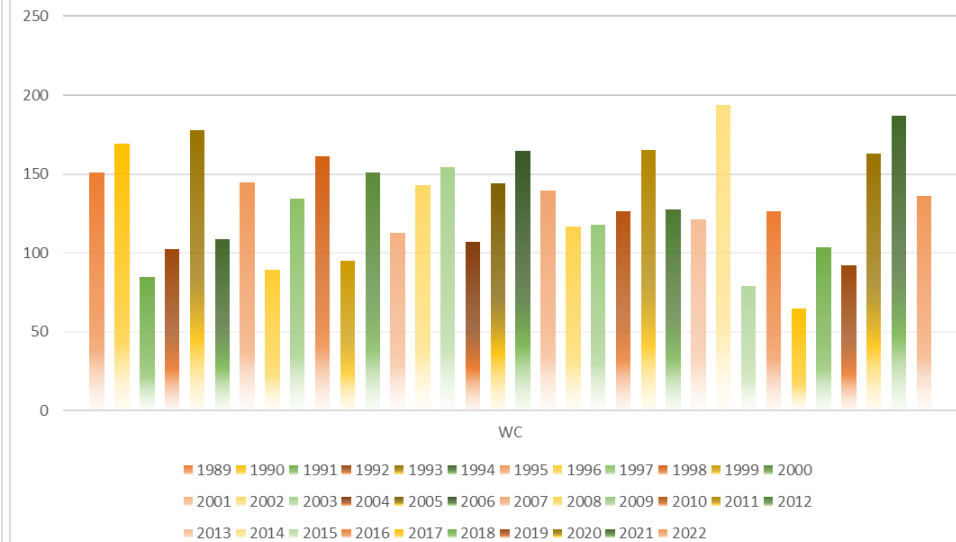
RAINFALL YEAR TO DATE WC
