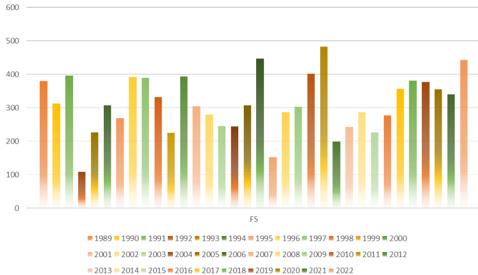
RAINFALL YEAR TO DATE FS
