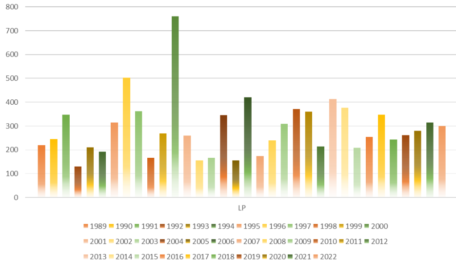
RAINFALL YEAR TO DATE LP
