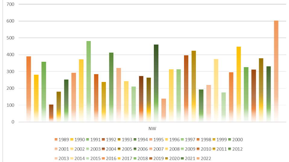
RAINFALL YEAR TO DATE NW
