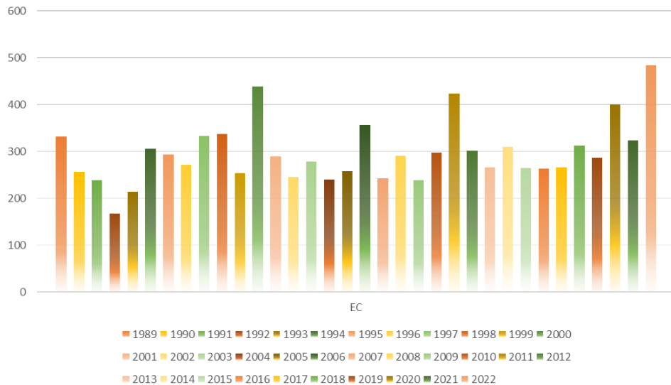
RAINFALL YEAR TO DATE EC
